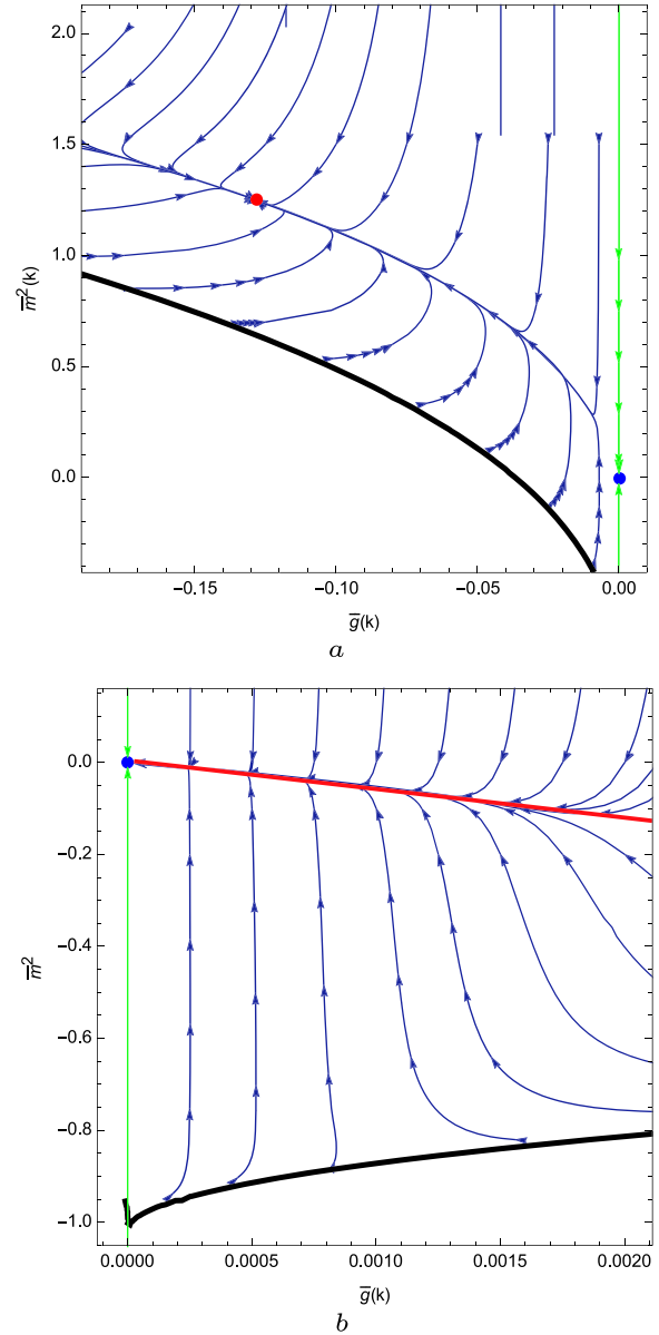
Fig. 2. The numerical renormalization group flow around the Gaussian fixed point, for \bar{g}(g) < 0 (a) and \bar{g}(k) > 0 (b). The blue point on both sides corresponds to the Gaussian fixed point, whereas the red point on (a) corresponds to the fixed point p_1 . The black line corresponds to the singularity \text{den} = 0 , and the green line corresponds to eigendirections of the Gaussian fixed point. Regular trajectories are pictured in blue.
