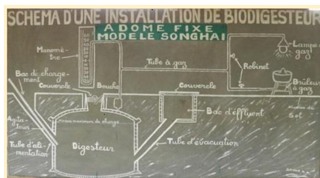
Figure 5: Diagram of a bio digester installation
