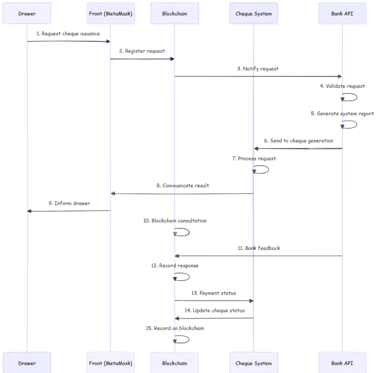
Fig. 7. Flow diagram of cheque generation process
