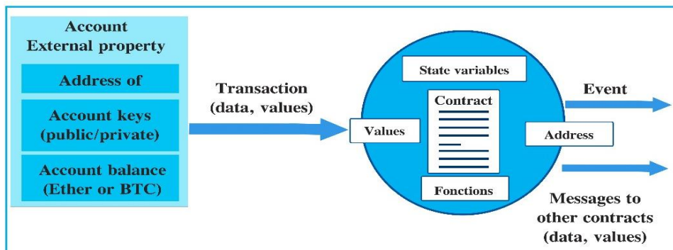
Fig. 3. How smart contracts work
