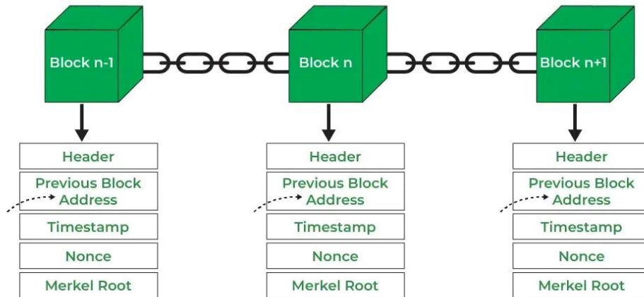
Fig. 2. The blockchain registry (GeeksforGeeks, 2022a)
