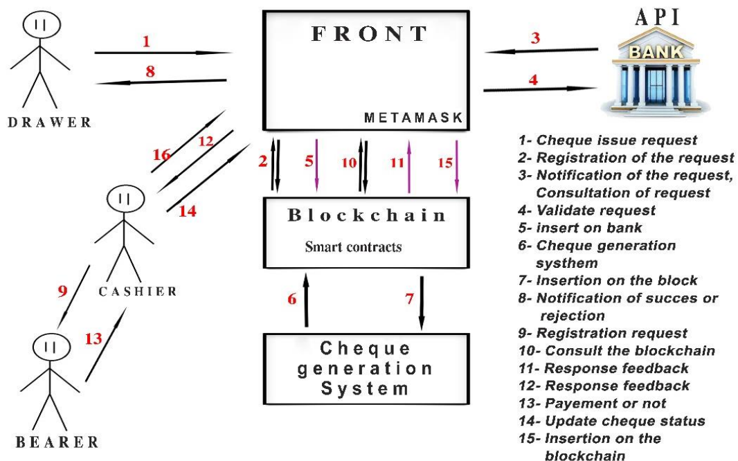
Fig. 6. System use case diagram
