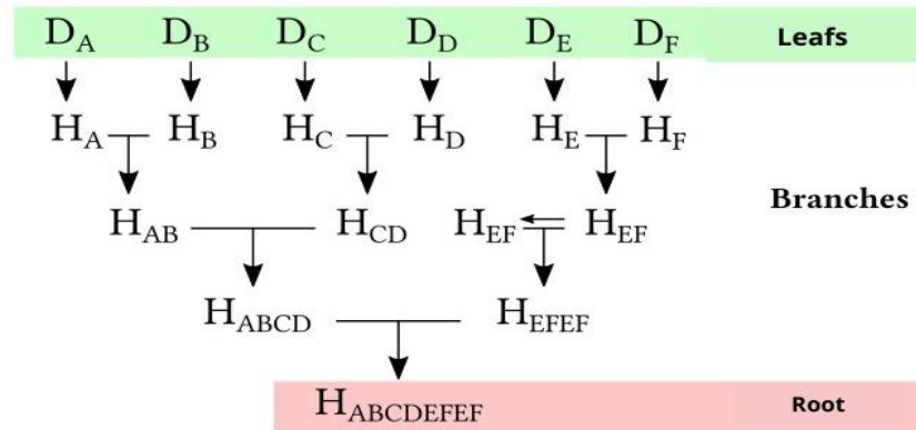
Fig. 5. Merkle tree (Lars, 2020)
