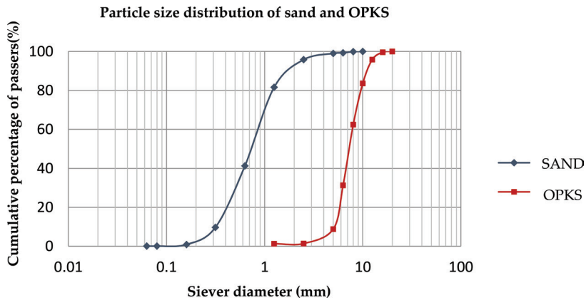
Figure 6. Particle size distribution of sand and OPKS.
