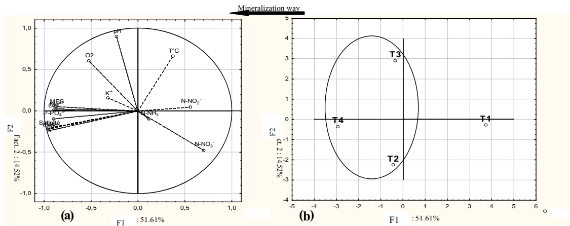
Fig. 2 Principal component analyses of treatments and their effect on water quality. a Correlation between chemical parameters; b classification of treatments
