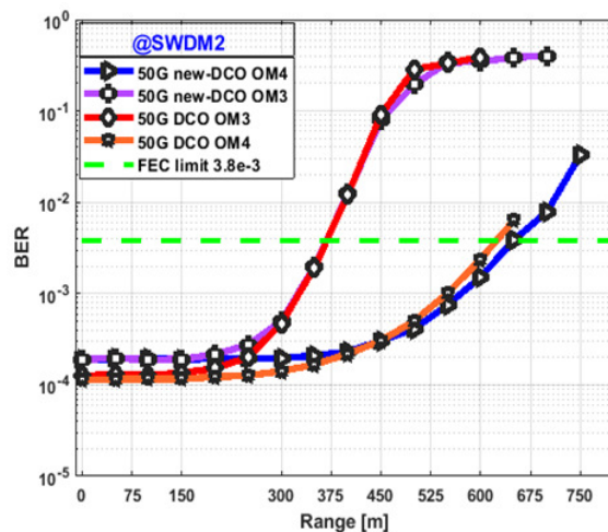
Fig.6 BER = f(Range) of the 100G-SWDM2 link with new-DCO-OFDM and conventional DCO-OFDM
