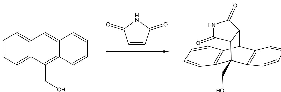
Figure 2. DA Benchmark reaction of anthracene-9-methanol with maleimide (for conditions, see Table 1)
