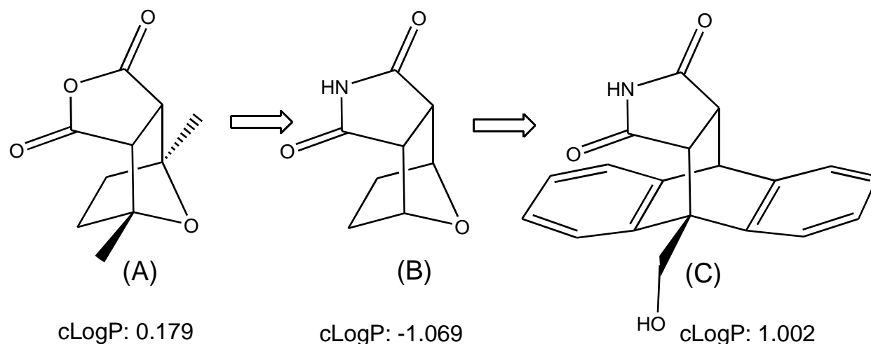
Figure 1. Design of cantharidine-like Structure C as trypanocidal lead
