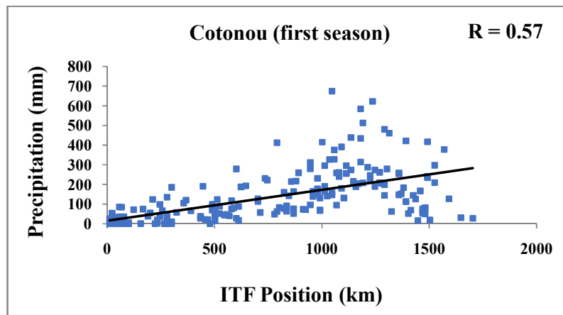
Fig. 10. Monthly precipitations in relation with the position of the ITF in accordance with the station of Cotonou (First season)
