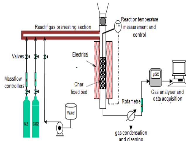
Figure 1: Diagram of the used experimental installation for gasification reactions of fixed bed type
