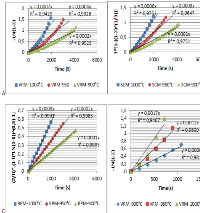
Figure 5: Plots of linearized VRM-SCC-RPM during gasification of corncobs char using respectively CO 2 (A, B and C) and steam (D, E and F) at 900 °C, 950 °C and 1,000 °C.
