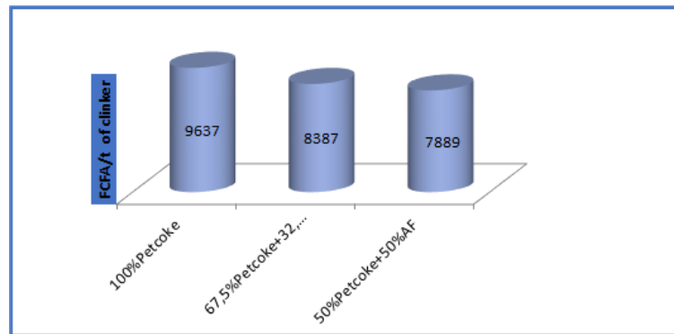
Fig. 5. Cost in CFAF/t of clinker as a function of the FA substitution rate.
